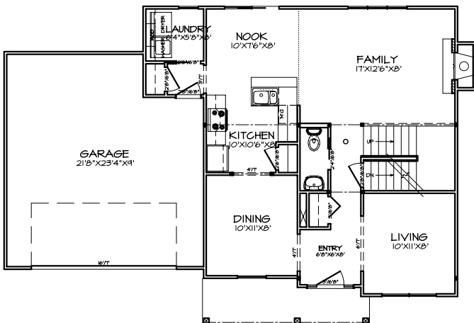
FIRST FLOOR PLAN A-4
