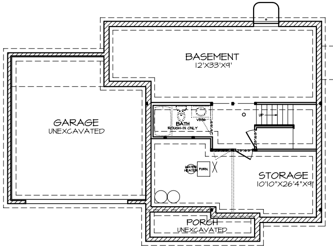
FOUNDATION PLAN A-3
