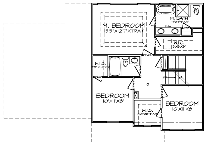
SECOND FLOOR PLAN A-5
